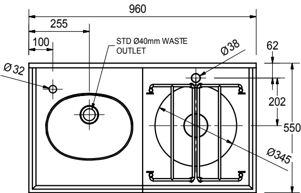
TOP VIEW LEFT HAND UNIT
