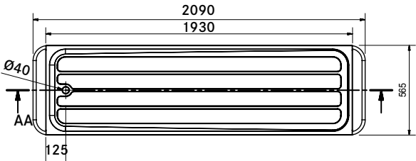
STANDARD PRESSED BODY TRAY - TOP VIEW
