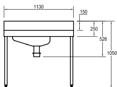
FRONT VIEW LEFT HAND BOWL
