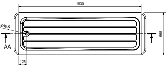
OBESE PRESSED BODY TRAY - TOP VIEW
