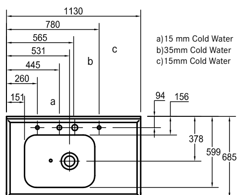
TOP VIEW LEFT HAND BOWL
