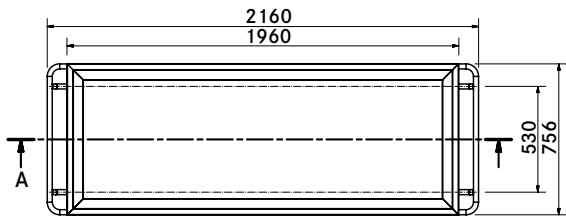
OBESE BTS BODY TRAY - TOP VIEW
