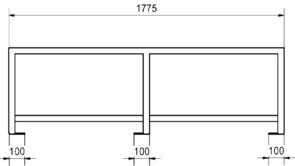
OPTIONAL BATH FRAME WITH LEGS
