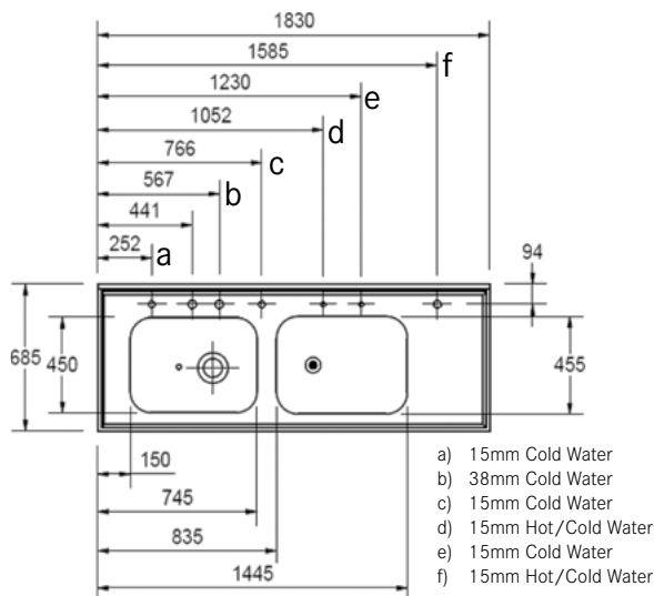
TOP VIEW LEFT HAND BOWL
