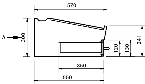
SECTION SIDE VIEW
