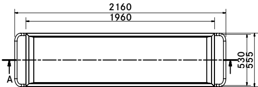
STANDARD BTS BODY TRAY - TOP VIEW
