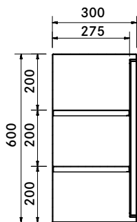
SECTION A -SIDE VIEW
