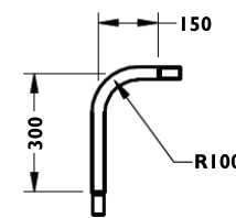
90° S/R BEND SW SHORT RADIUS
