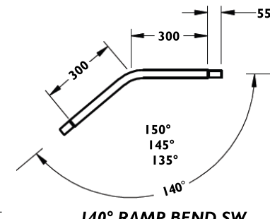
140° RAMP BEND SW
