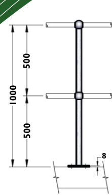
90° TM TOP MOUNT
