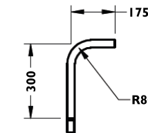
90° T/R BEND SW TIGHT RADIUS STAIR RETURN BENDS
