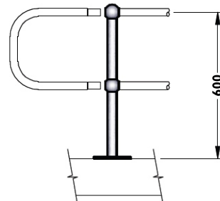
2-BALL 600 STANCHION C/W 300 CLOSURE
