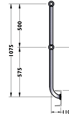
90° GN GOOSE NECK STD 110MM OFFSET PLEASE SPECIFY 140mm OFFSET
