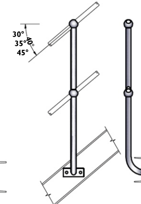
40° GN L/R GOOSE NECK STD 110mm OFFSET PLEASE SPECIFY 140mm OFFSET & LEFT OR RIGHT
