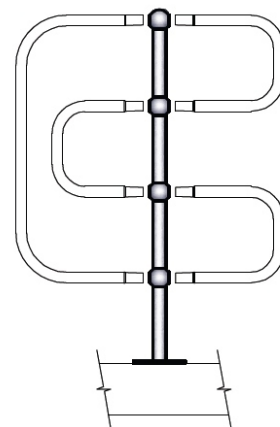
4-BALL STANCHION C/W 750 CLOSURE & 250 CLOSURE
