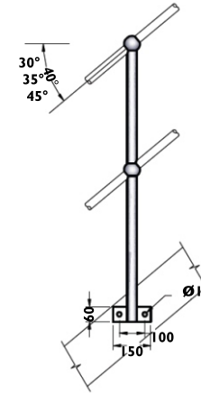
40° SM L/R SIDE MOUNT PLEASE SPECIFY LEFT OR RIGHT
