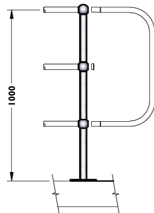
3-BALL STANCHION C/W 666 CLOSURE & 38mm PLASTIC END PLUG
