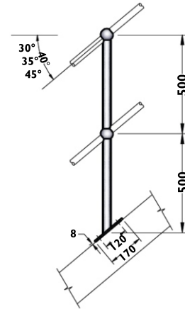
40° TMA TOP MOUNT ANGLE BASE
