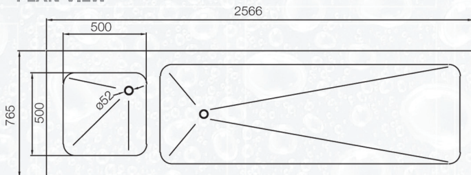
PLAN VIEW
