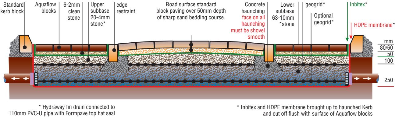
Tanked system section: Aqua pavement with undersealing membrane
