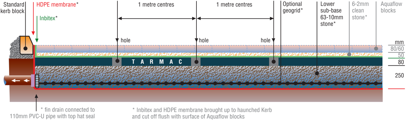
Tanked system section: Aquaflow pavement with undersealing membrane
