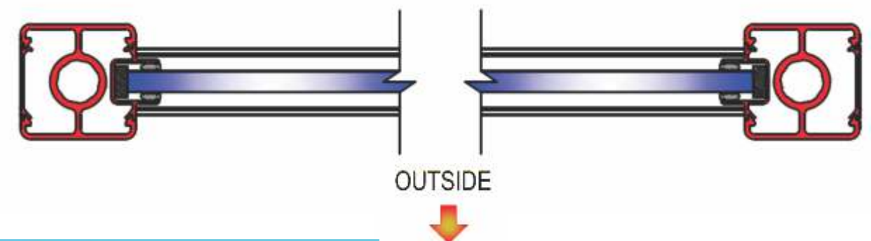
SECTION B-B
