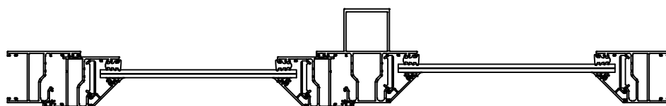
Section B-B
