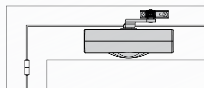
Installation on hinge side
