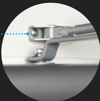
EN standard force adjusted by changing the position of the support (see Installation Instructions)
