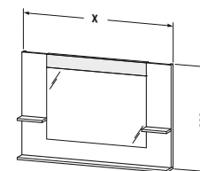
# VE 7350 ↔ 850 mm ⌀ 1 x 11 W # VE 7351 ↔ 1000 mm ⌀ 1 x 14 W # VE 7352 ↔ 1200 mm ⌀ 1 x 18 W # VE 7353 ↔ 1400 mm ⌀ 1 x 22 W # VE 7354 ↔ 1600 mm ⌀ 1 x 28 W ↗ 142 mm IP 44 LED A++
