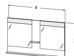
# VE 7360 ↔ 1150 mm ⌀ 1 x 22 W # VE 7361 ↔ 1400 mm ⌀ 1 x 28 W # VE 7362 ↔ 1800 mm ⌀ 1 x 36 W # VE 7363 ↔ 2000 mm ⌀ 1 x 36 W ↗ 142 mm IP 44 LED A++
