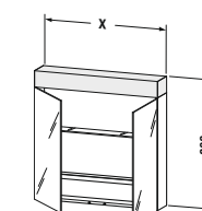
# VE 7501 ↔ 600 mm ⌀ 1 x 11 W # VE 7502 ↔ 800 mm ⌀ 1 x 14 W # VE 7503 ↔ 1000 mm ⌀ 1 x 18 W ↗ 142 mm IP 44 LED A++
