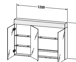
# VE 7504 ⌀ 1 x 22 W ↗ 142 mm IP 44 LED A++
