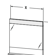
# VE 7300 ↔ 450 mm ⌀ 1 x 11 W # VE 7301 ↔ 600 mm ⌀ 1 x 14 W # VE 7302 ↔ 800 mm ⌀ 1 x 18 W # VE 7303 ↔ 1000 mm ⌀ 1 x 22 W # VE 7304 ↔ 1200 mm ⌀ 1 x 28 W ↗ 142 mm IP 44 LED A++
