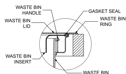
DETAIL 1
