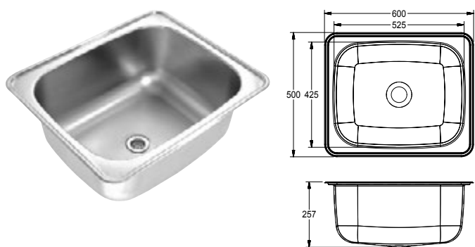
DLT Luxtub - Inset Type Wash Trough
