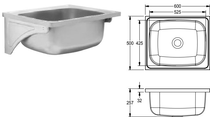
LDL Lux Tub - Wall Mounted/Drop-On Wash Trough
