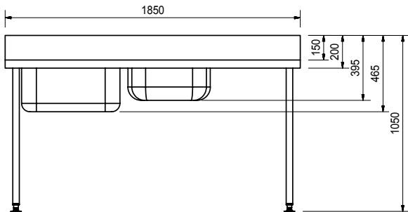
LEFT HAND BOWL FRONT VIEW
