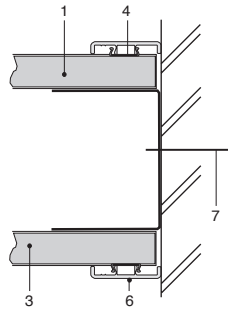
A) Wall abutment detail
