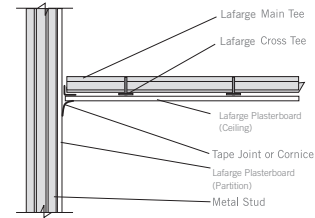
Finished joint between wall and ceiling
