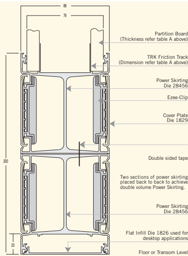
Power Skirting accessories as per Crabtree and Clipsal 2000 series range.
