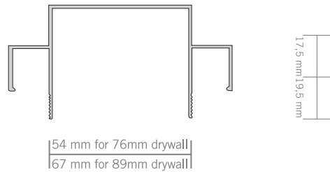
Female Recessed Head Die 6165 for 76mm / Die 6166 for 89mm
