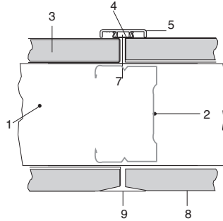
B) Jointing of boards
