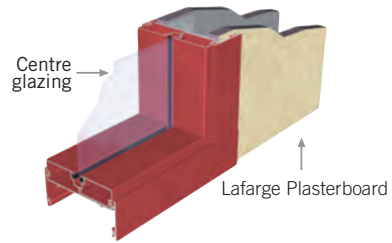
Main Post showing partition board and centre glazing details.
