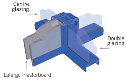
4 Way Box Post showing partition board and full height glazing details.
