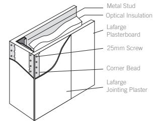
External Corner Fair End Concealing
