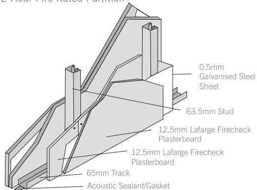
2 Hour Fire Rated Partition
