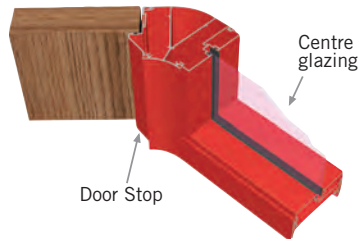
135V45Y corner post showing Door Stop and Centre Glazing details.
