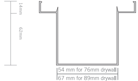
Female Recessed Base Die 6206 for 76mm / Die 6207 for 89mm
