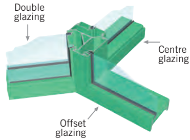
3 Way Y Post showing three different floor glazing details.
