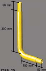
ITEM 20 Standard 90° Short Radius Bend (mass 0.9kg)
