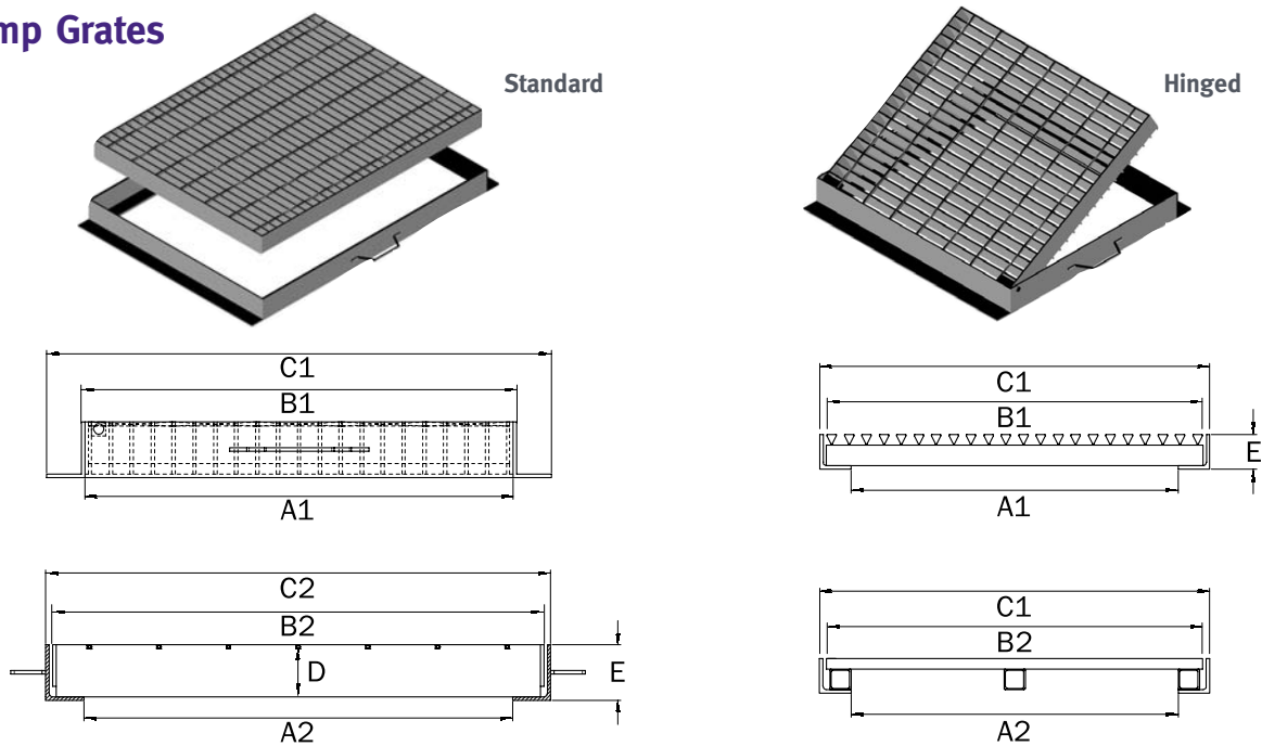
Ezi - Walk Class A
