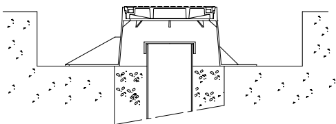
DCC4D32 Concrete encasement not required
