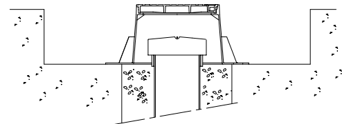
DCC3B32 Concrete encasement not required
