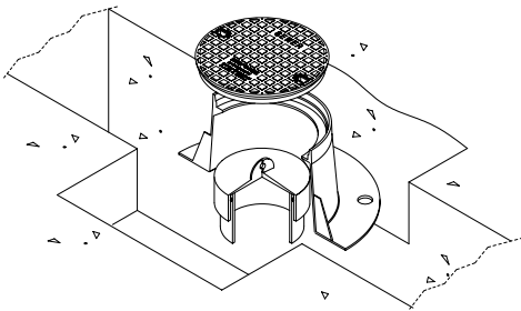
DCC3B32 Concrete encasement not required
