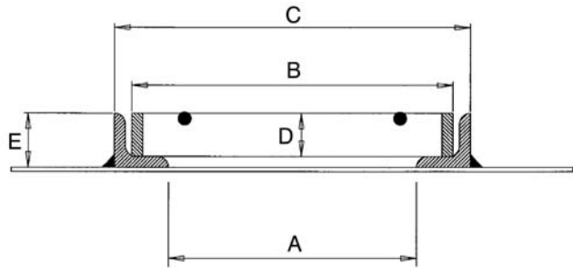
Standard Grating Class B, C & D
