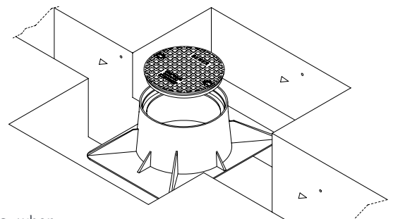
DCC4D32 Concrete encasement not required
