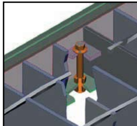
Holding down bolts to prevent unauthorised entry
